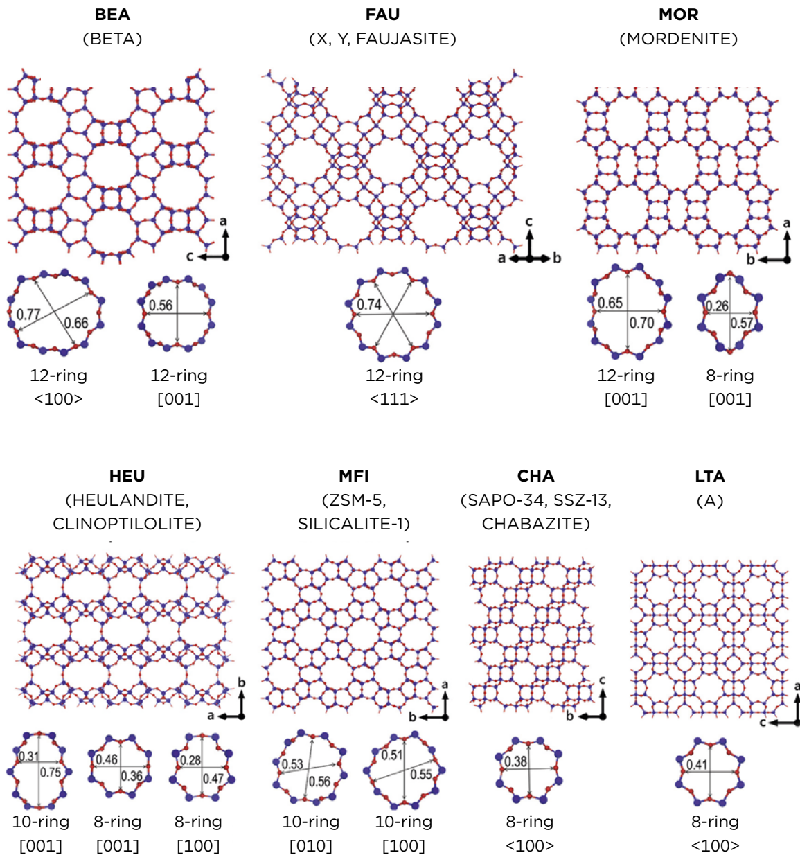
Figure 1. Common zeolite frameworks, showing for each type: three-letter IZA code, zeolite names, framework structure (blue: T atoms, red: oxygen), and pore windows with size (nm) and direction. [Source: 2. Li, et al.]
